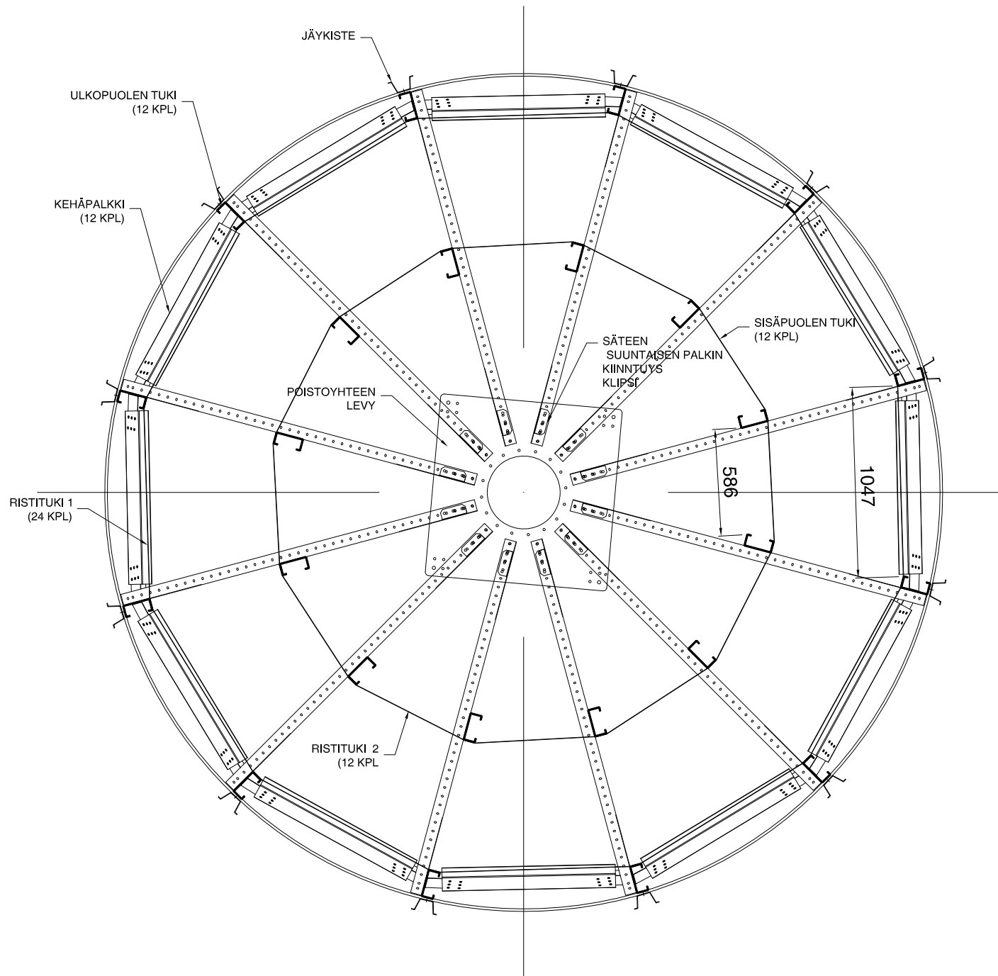
STRUCTURE Ø460 T30 (TYPE 2)
