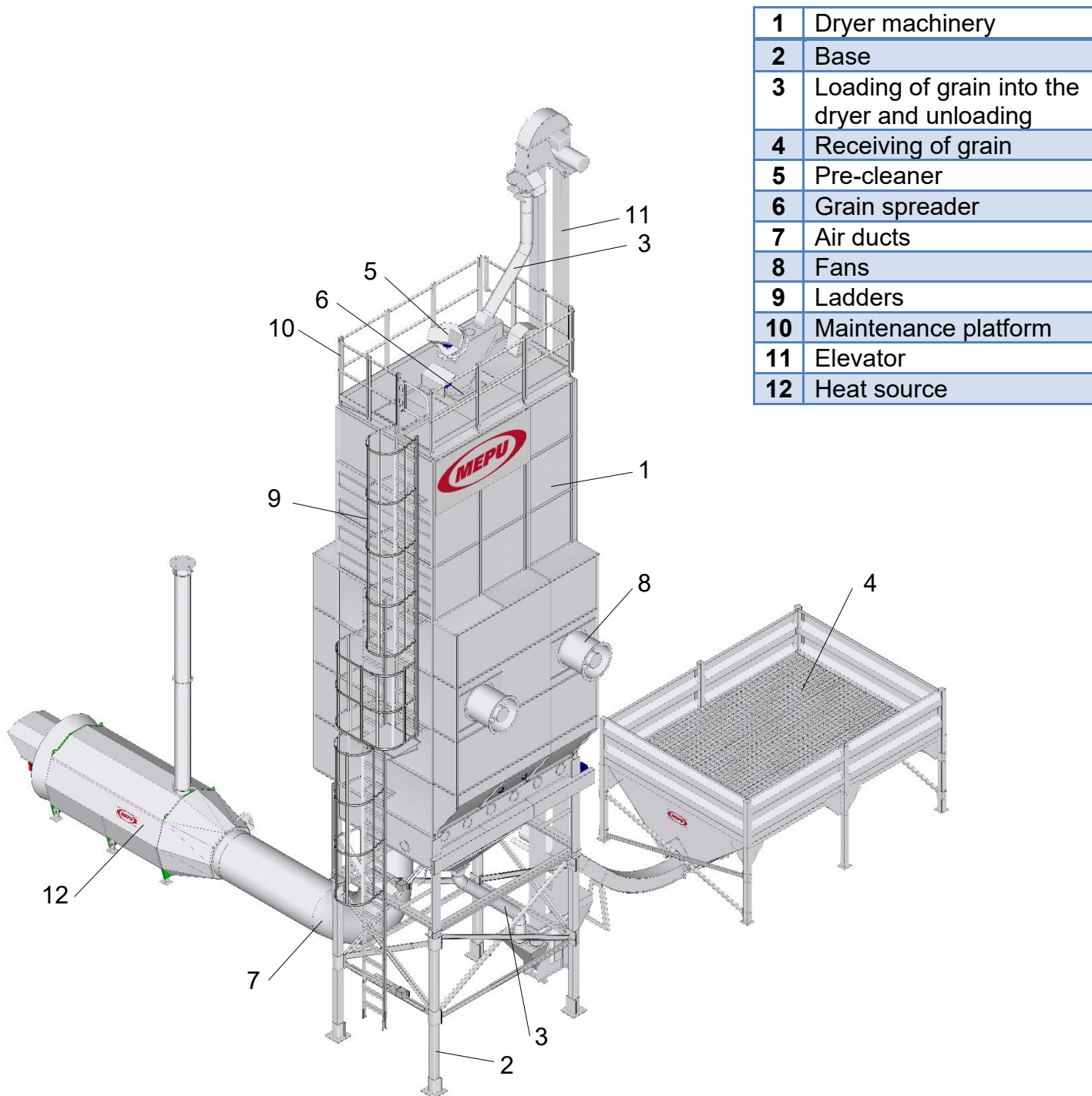
Figure 1. Key parts of a grain dryer
