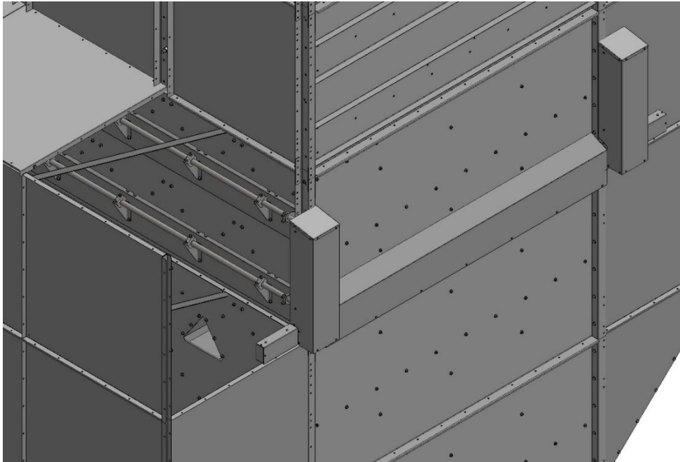
Figure 13. Air casing adjustment shutter (electrical).
