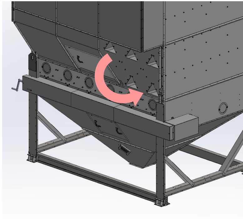
Figure 11. Return of kernels from the air casing.
