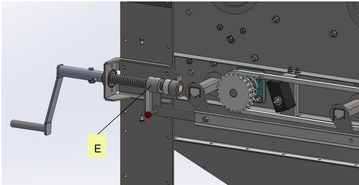
Figure 8. Maintenance points of the feeding apparatus (bottom hatches' drive unit side).
