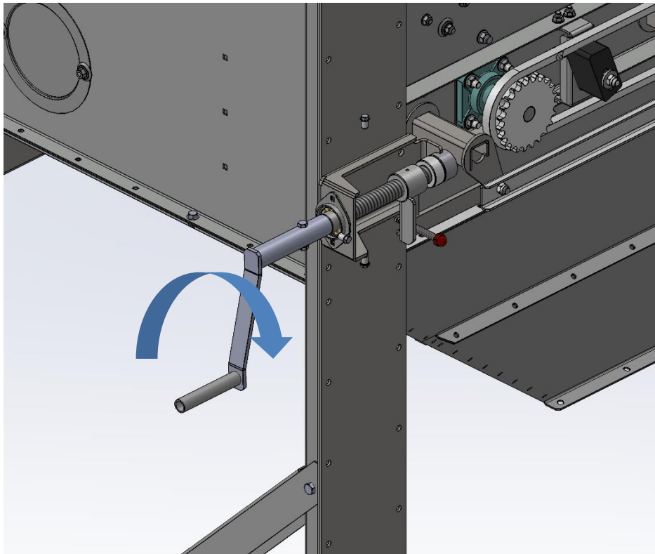
Figure 5. Closing the bottom hatches.
