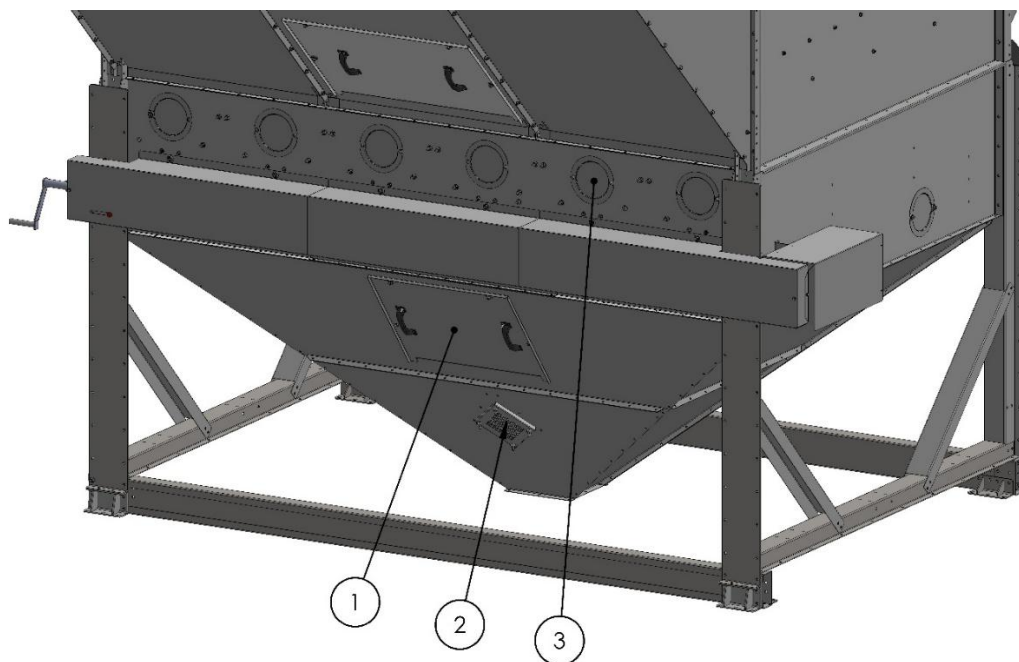
Figure 10. Bottom cone.
