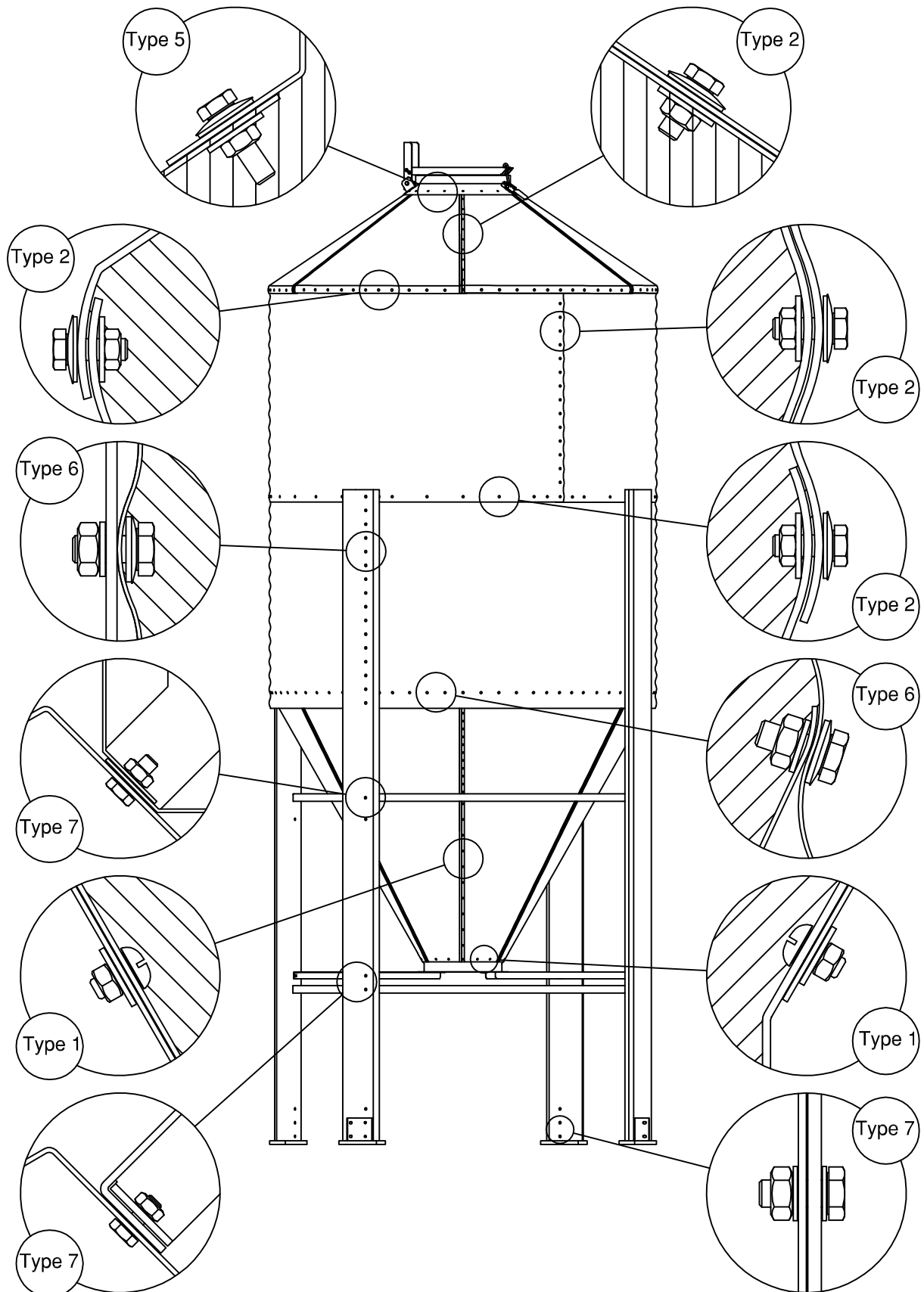
Types of joint shown by their different positions. Bolts, nuts and washers specifications.
