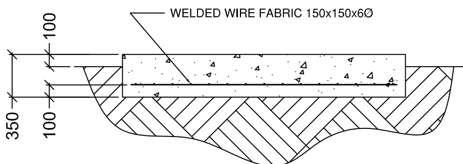
FOUNDATION CROSS SECTION
