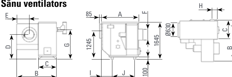
Sānu ventilators
